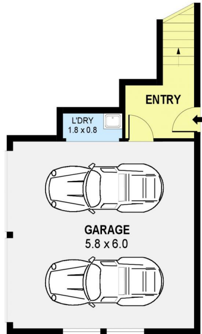
GROUND LEVEL
